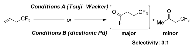
Scheme 3. Influence of inductive effects on the regioselectivity of the Wacker oxidation of terminal alkenes. Quantitative conversion relative to BQ was observed. DMF = N,N -dimethylformamide. Conditions A (Tsuji–Wacker): [Pd(PhCN) 2 Cl 2 ] (5 mol%), BQ (1.0 equiv), DMF/H 2 O (7:1), 40 °C, 16 h; conditions B (dicationic Pd): Pd(OAc) 2 (7.5 mol%), BQ (1.0 equiv), MeCN/H 2 O (7:1), HBF 4 (0.27 M), 40 °C, 16 h.
